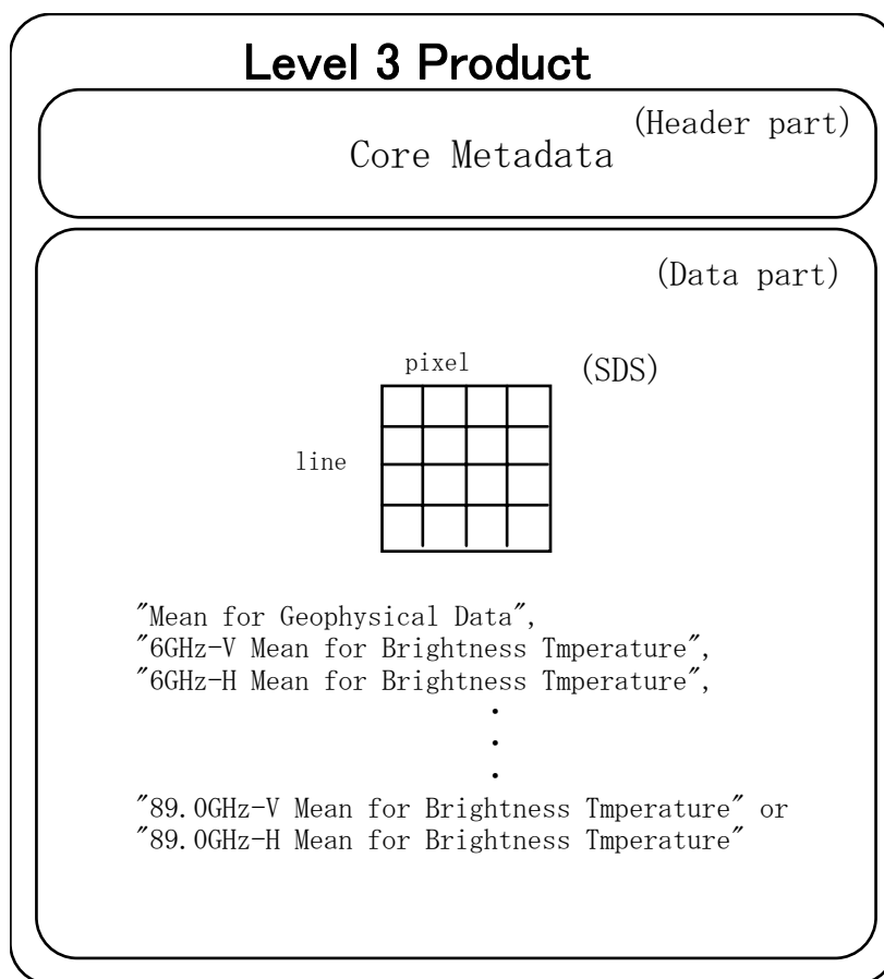
Figure 3-1 Structure of level 3 product.
