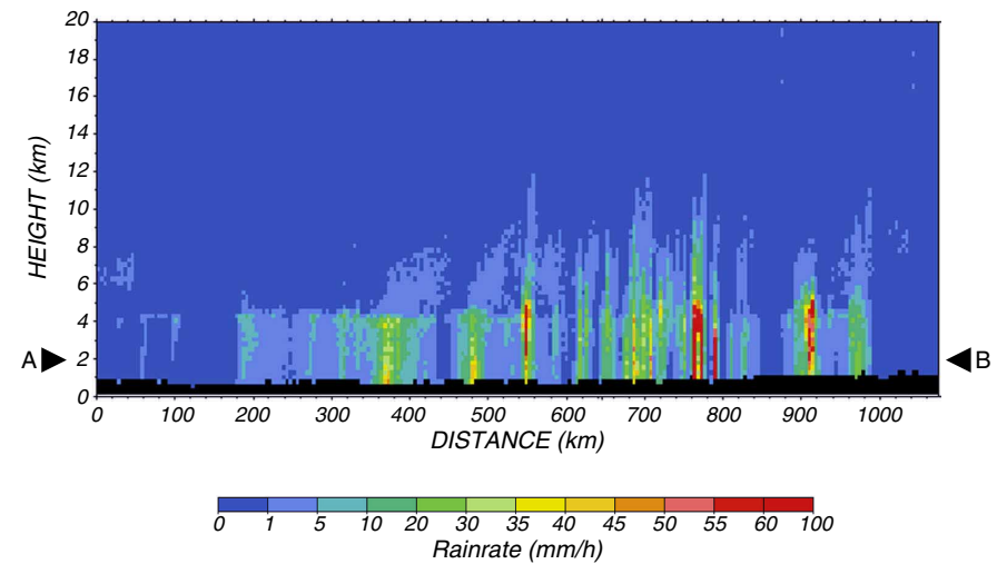
Fig.4 PR: Vertical Cross Section
