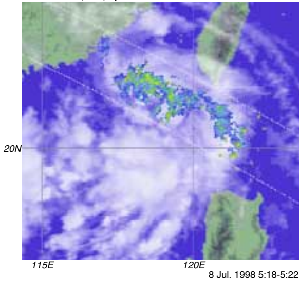
GNS IR 5:00 (UTC) by JWA
