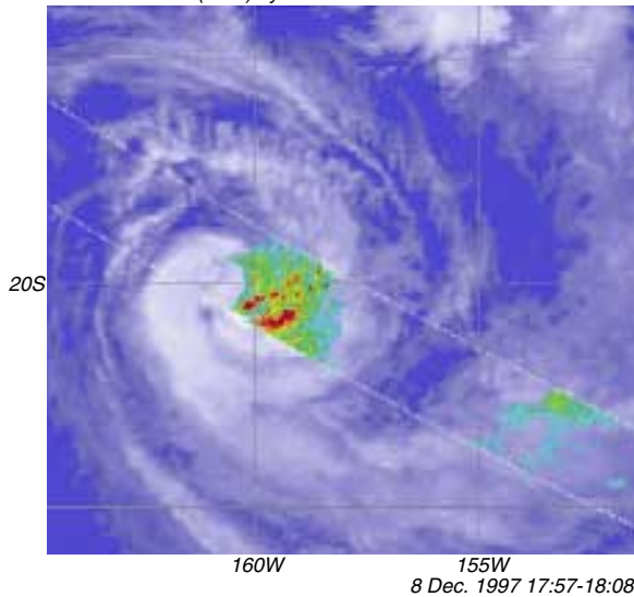
GOES IR 18:00 (UTC) by JWA
