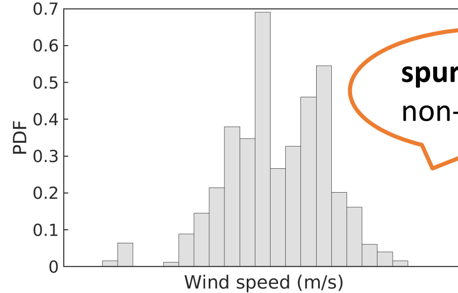
surface wind probability distributions
