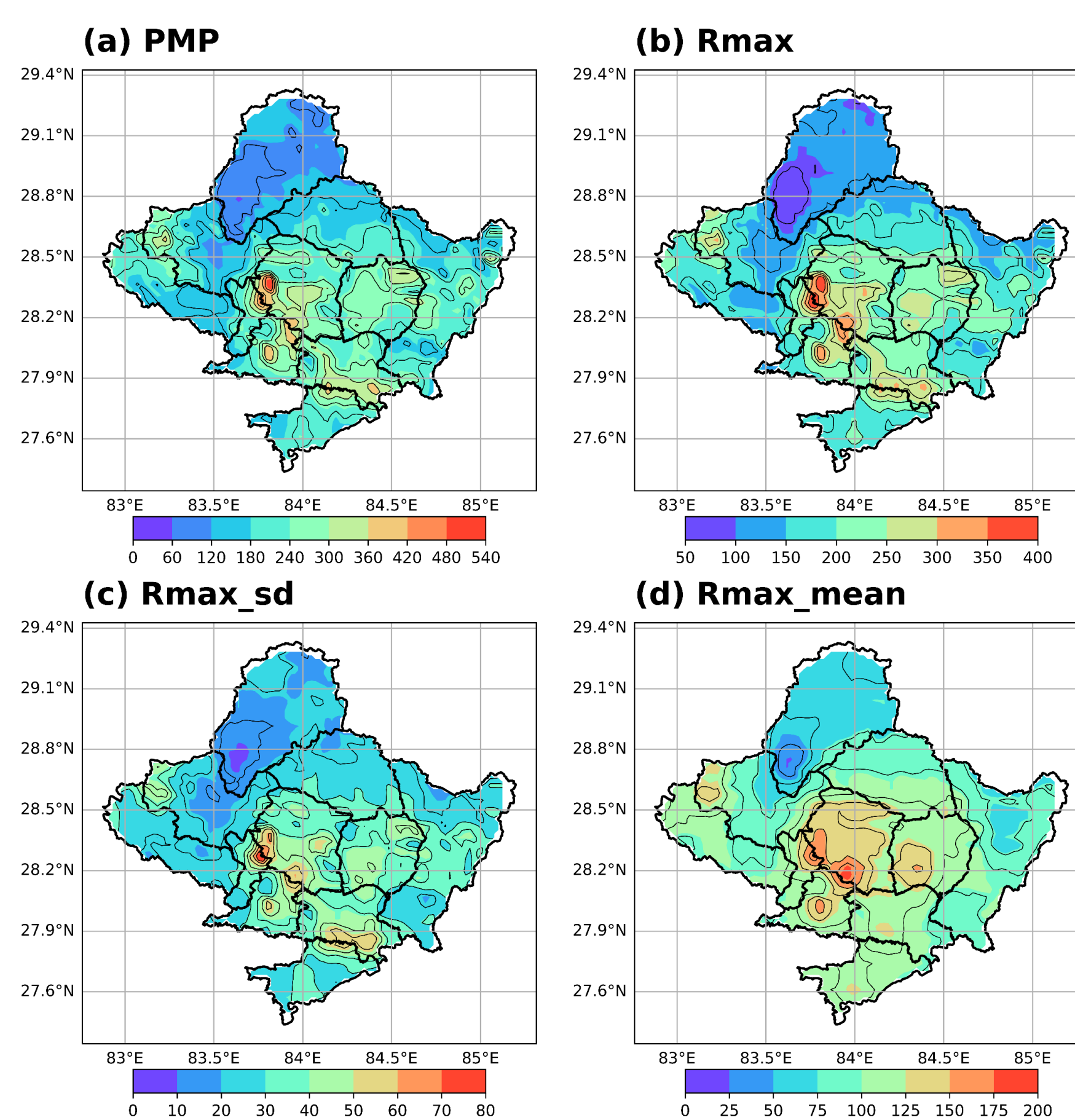
Figure 6: (a) Probable Maximum Precipitation computed using Hershfield technique (Hershfield, 1961) (PMP; mm/day), (b) 31-year maximum precipitation (Rmax; mm/day), (c) maximum precipitation standard deviation (Rmax_sd; mm/day), and (d) maximum precipitation mean (Rmax_mean; mm/day). The climatology was examined using the 5-kilometer CHIRPS precipitation dataset from 1992 to 2022.
