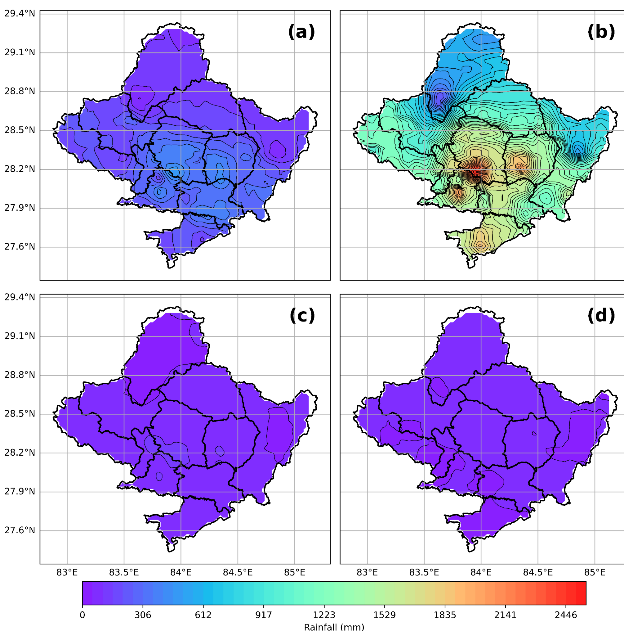
Figure 2: Seasonal accumulated precipitation, (a) Pre-monsoon, (b) Monsoon, (c) Post-monsoon, and (d) Winter. The climatology was examined using the 5-kilometer CHIRPS precipitation dataset from 1992 to 2022.
