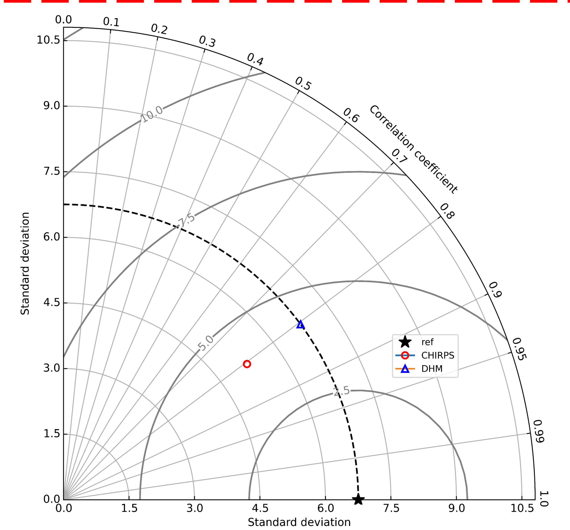
Figure 1: Taylor diagram indicating daily climatology's standard deviation, correlation coefficient, and centered root mean square error from 1992-2022.
