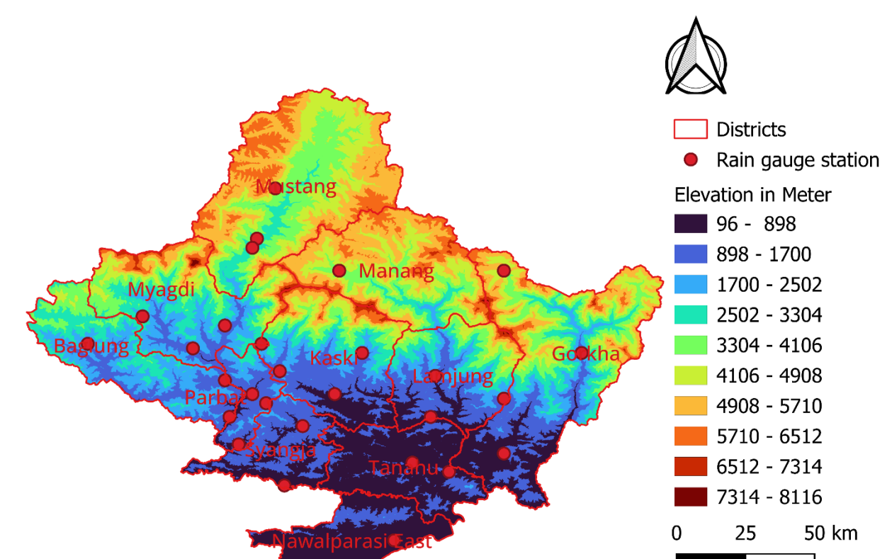
Figure 8: Spatial distribution of rain gauge stations and elevation in the study area.
