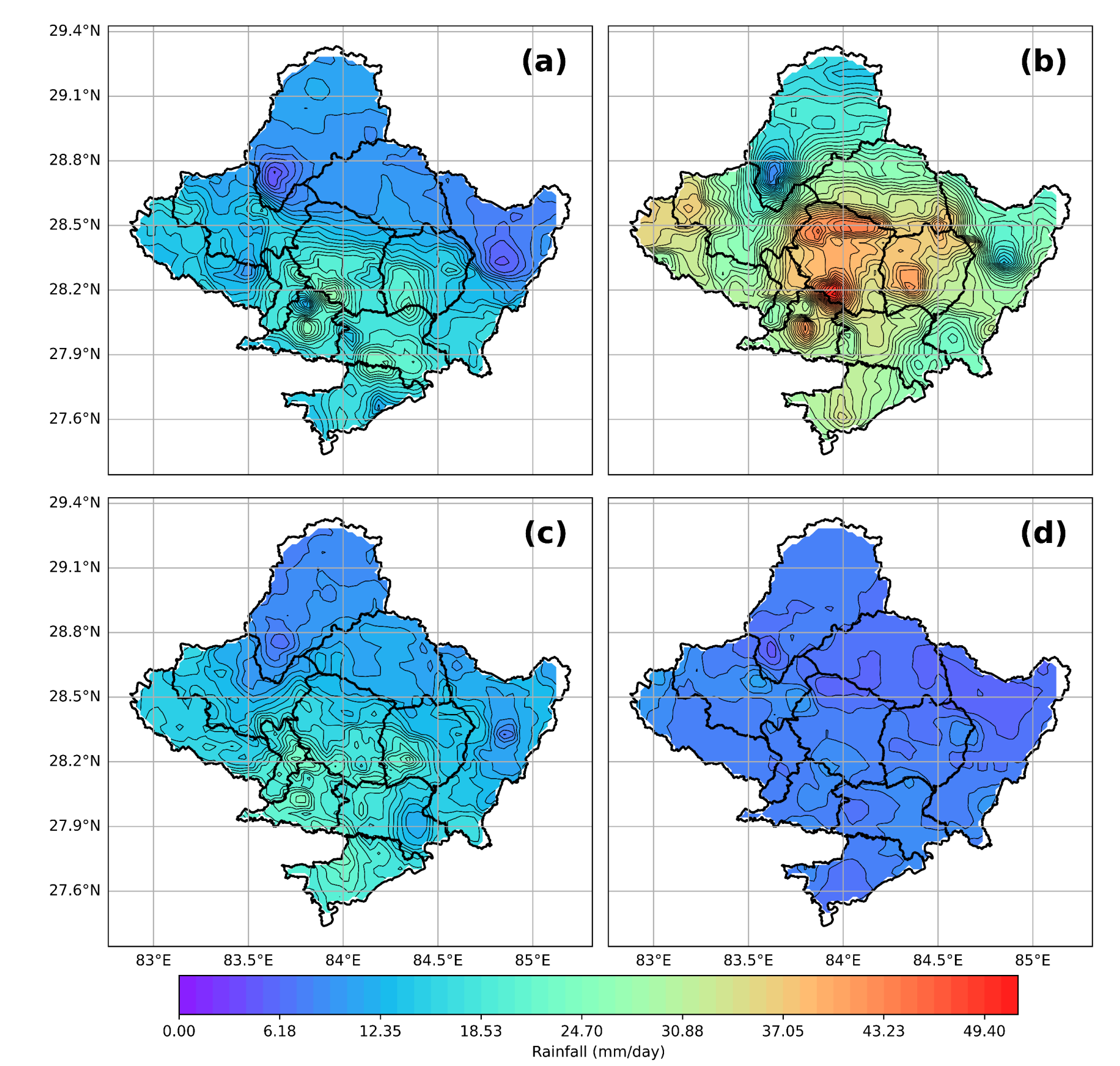
Figure 4: Seasonal rainfall intensity, (a) Pre-monsoon, (b) Monsoon, (c) Post-monsoon, and (d) winter. The climatology was examined using the 5-kilometer CHIRPS precipitation dataset from 1992 to 2022.
