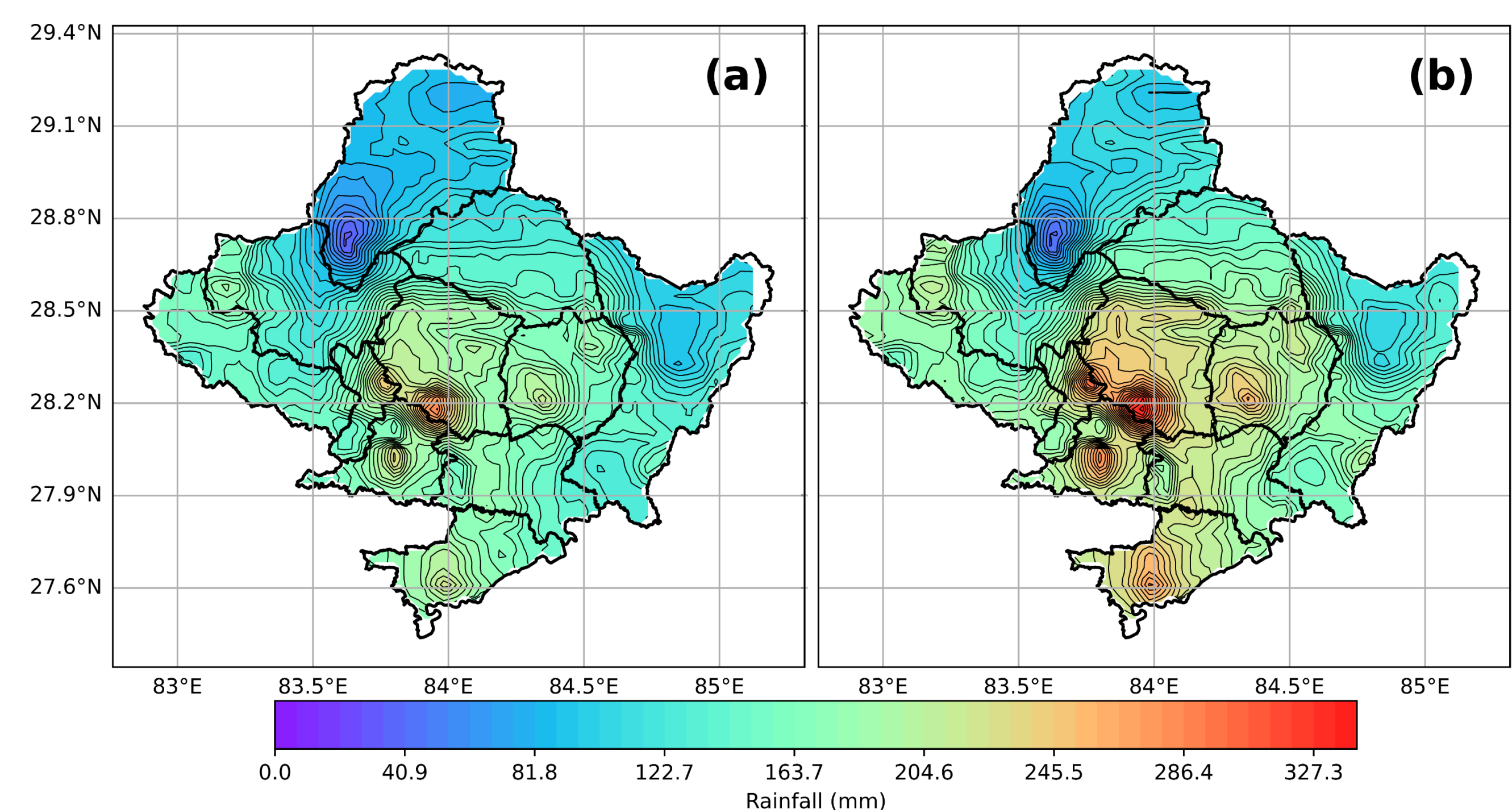
Figure 5: (a) 3-day maximum precipitation and (b) 5-day maximum precipitation. The climatology was examined using the 5-kilometer CHIRPS precipitation dataset from 1992 to 2022.
