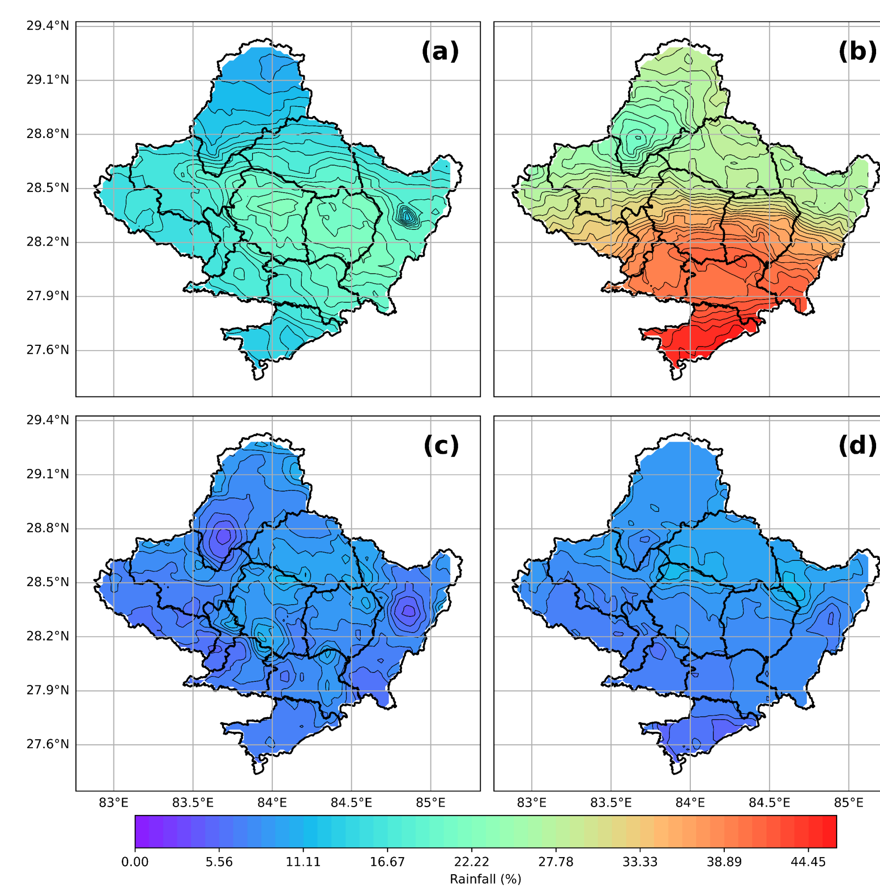
Figure 3: Seasonal rainfall frequency of days greater than or equal to 1mm per day, (a) Pre-monsoon, (b) Monsoon, (c) Post-monsoon, and (d) winter. The climatology was examined using the 5-kilometer CHIRPS precipitation dataset from 1992 to 2022.
