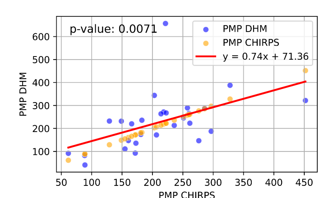
Figure 7: Scatter plot comparing (PMP) values between CHIRPS and DHM datasets.
