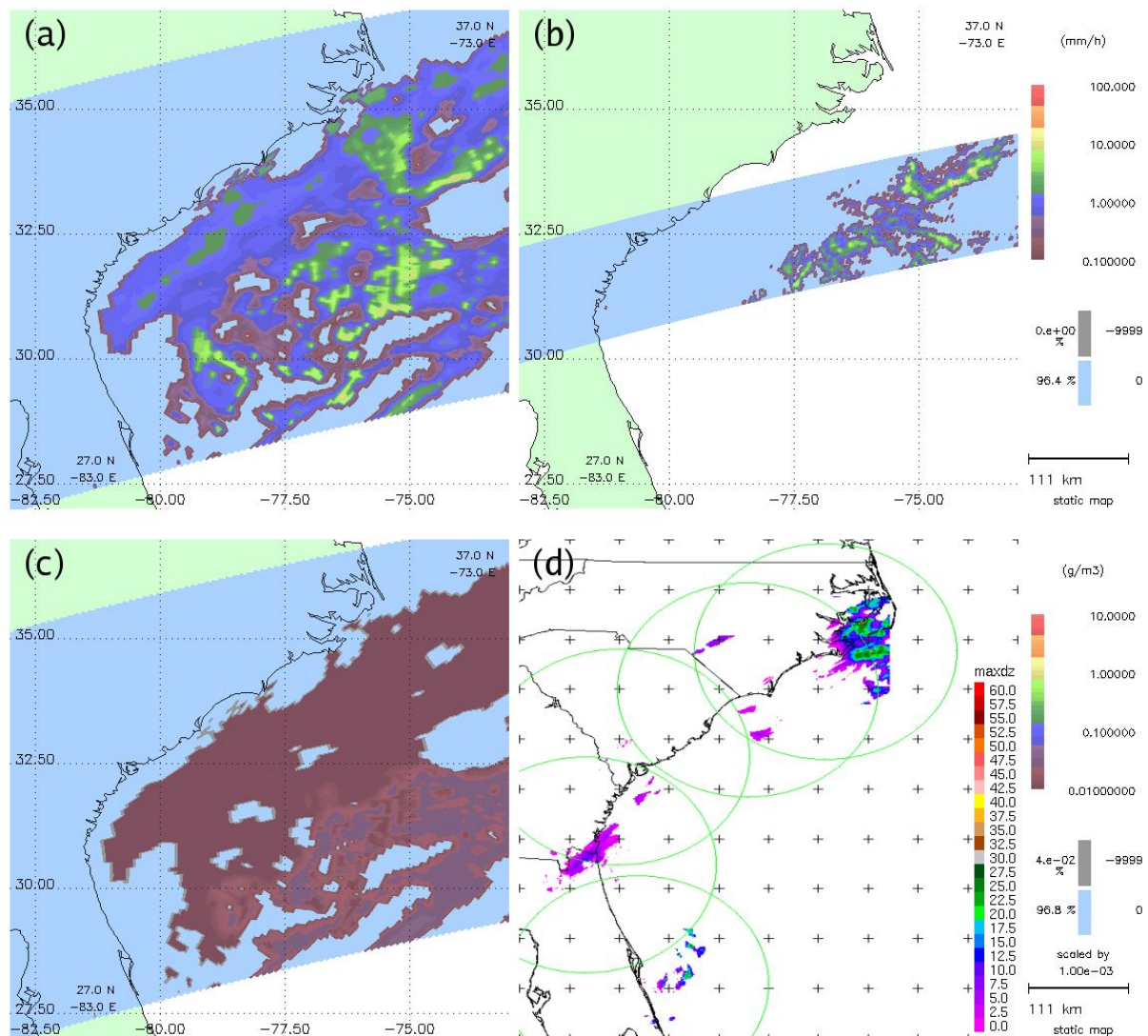
Figure 5. Phantom precipitation off the Atlantic Coast of the southeastern US on 18 March 2005. (a) TMI surface precipitation retrieval. (b) PR near surface precipitation. (c) 14km TMI cloud ice above observed cloud top level. (d) Coastal S-band radar composite. Rings denote maximum range.
