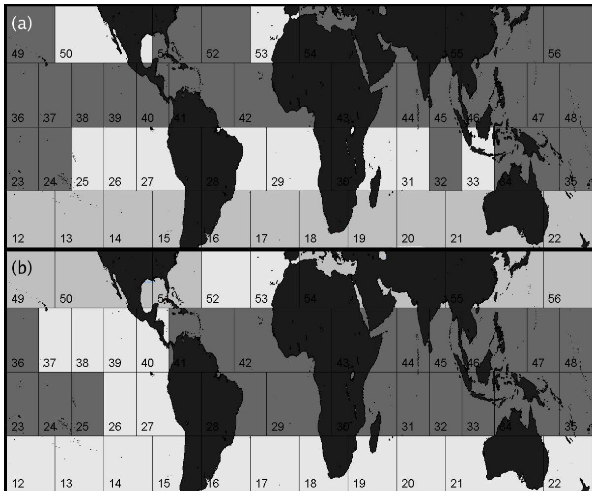
Figure. 2. Map of oceanic regional PDF shape for 47 day accumulated V6 TMI instantaneous rain rates. Color coding indicates unimodal (medium grey), bimodal (dark grey), and strongly skewed (light grey) distributions in \log_{10}(R) . (a) Northern Hemisphere (NH) summer from 16 June – 1 August 2001. (b) NH winter from 1 Jan – 16 Feb 2002. Grid numbers are in lower left corner of each grid box.
