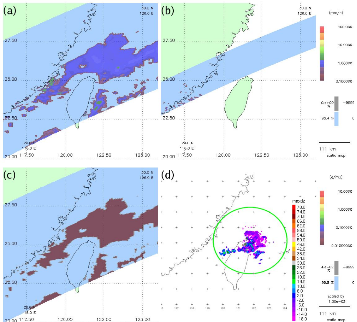
Figure 6. Phantom precipitation off the Taiwan coast on 1 Feb. 2000. (a) TMI surface precipitation retrieval. (b) PR near surface precipitation. (c) 14km TMI cloud ice above observed cloud top level. (d) Coastal S-band radar composite. Ring denotes maximum range.
