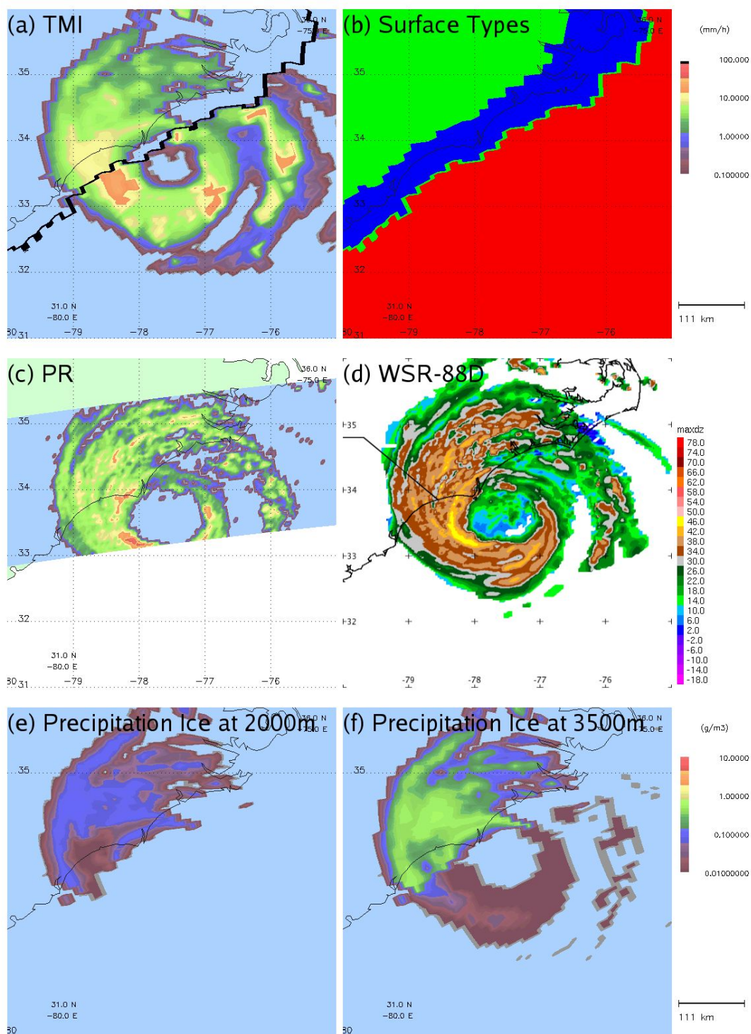
Figure 4. Views from different sensors of Hurricane Ophelia straddling the North Carolina coast at ~1400 UTC on 14 September 2005. (a) TMI precipitation retrieval with coast/ocean surface border overlaid. (b) Surface masked used in 2A-12: land, coast, and ocean. (c) PR near surface precipitation. (d) Combined radar reflectivity from coastal NWS WSR-88D radars at Morehead City, NC and Wilmington, NC. (e) TMI precipitation ice at 2000 m about the surface. (f) TRMM 2A-25 precipitation ice at 3500 m above the surface.
