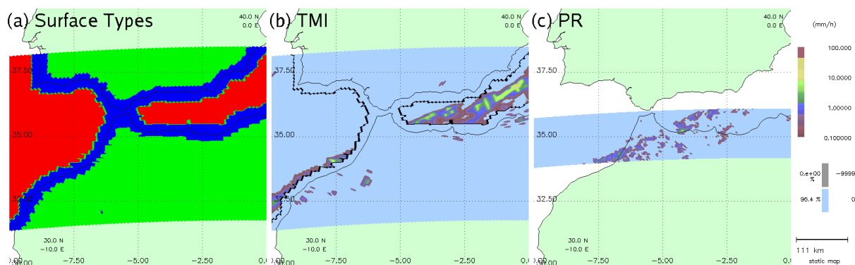
Figure 3. Shallow precipitation along the northern Morocco coast on 19 September 1999. (a) Surface masked used in 2A-12: land, coast, and ocean. (b) TMI precipitation retrieval with coast/ocean surface border overlaid. (c) PR near surface precipitation.
