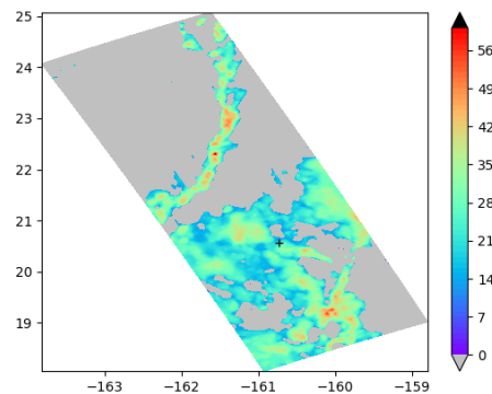
pyplot.contourf
