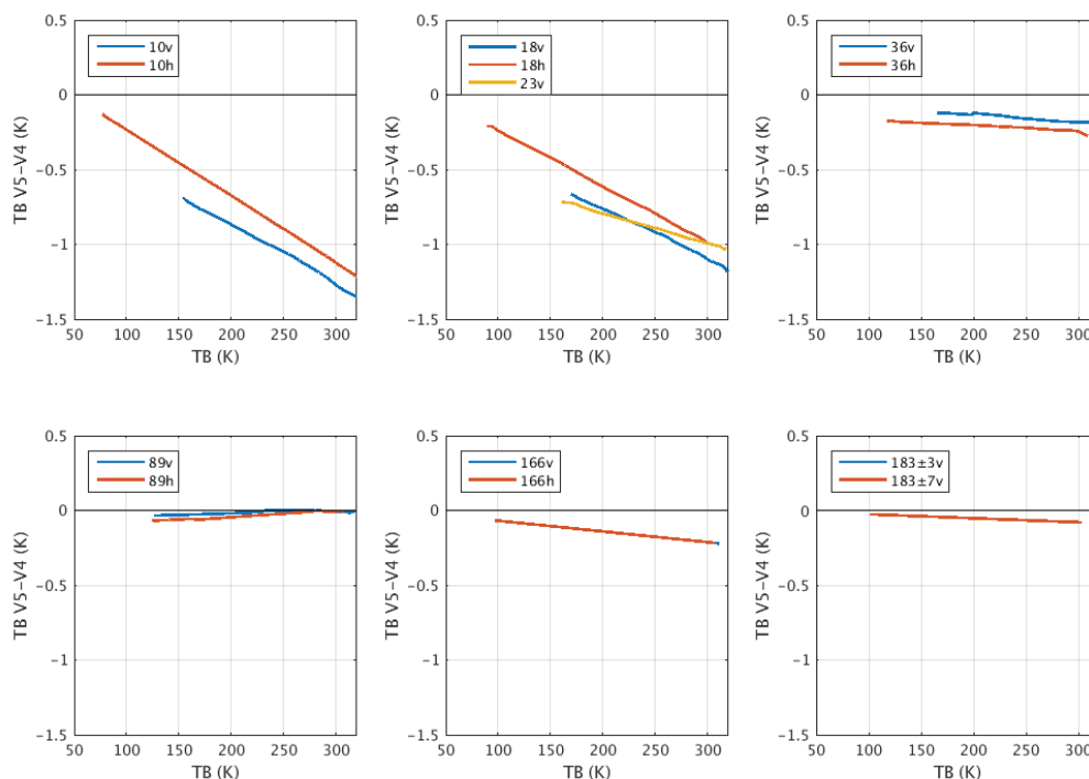
Figure 1. GMI T_b changes from V04 to V05.
