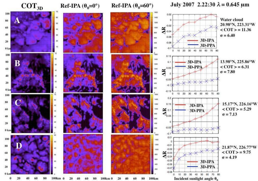
Fig. 4.4.4. Four scenes of 100kmx100km areas reconstructed by the MIDPM. Distributions of the Cloud Optical Thickness (COT) and flux reflectivity by the Independent Pixel Approximation (IPA) for two solar zenith angles \theta_0 = 0^\circ and 60^\circ . Right column panels shows the dependence of the difference between reflectances by MCstar and IPA or Plane Parallel Approximation (PPA) on the incident solar zenith angle \theta_0 .
