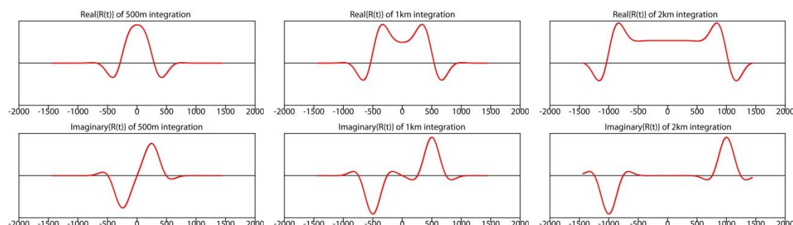
Fig. 3.1.3.1.1.2 Horizontally integrated C(X_E) and Q(X_E) in case of 500m (left), 1km (middle), 2km (right) integration
