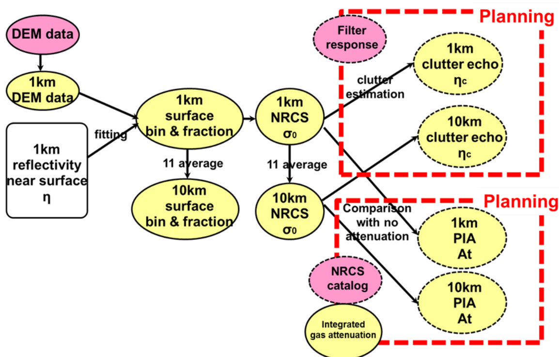
Figure 3.1.1.2.1-4 Processing flow of 1-km and 10-km averaged surface information
