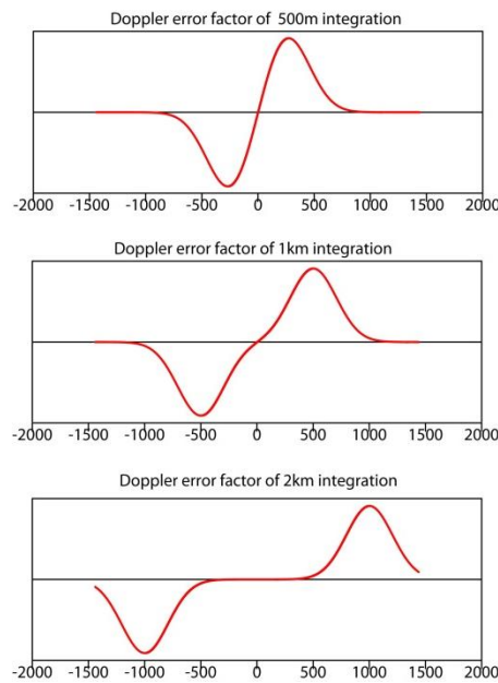
Fig. 3.1.3.1.1.1 Doppler error contribution factor in case of 500m (top), 1000m (middle), 2000m (bottom) integration
