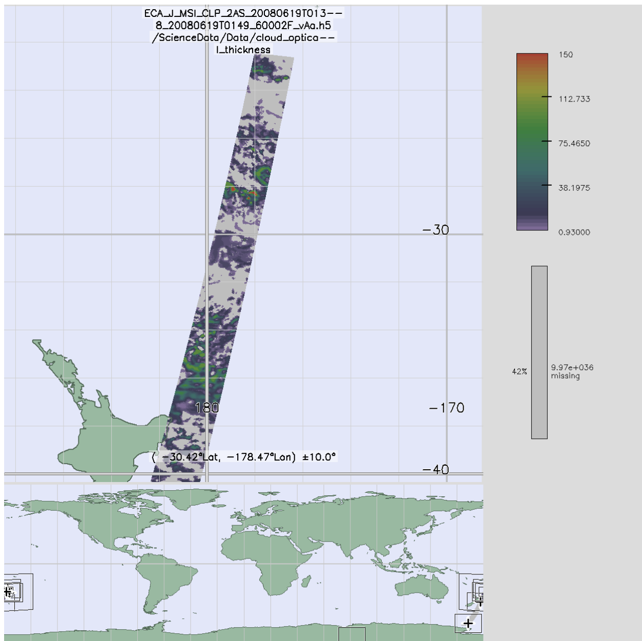
Fig.3.3.2.2.1.1 A sample of cloud optical thickness from L2A cloud product, which contains both water and ice clouds.
