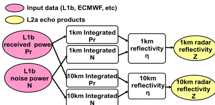
Figure 3.1.1.2.1-3 Processing flow of 1-km and 10-km averaged radar reflectivity
