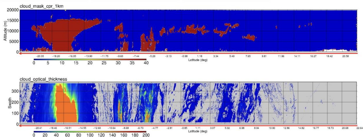
Fig.3.3.2.2.1.3 A sample of CPR cloud flag (upper) and MSI cloud optical thickness, monitoring a typical tropical cyclone in Indian Ocean on Jan.30, 2025 (03834E).
