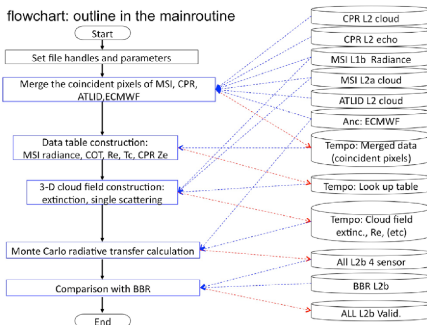
Figure 4.4.2. A flow chart of the 4 sensor radiative flux estimates with 3D RTM and MIDPM.
