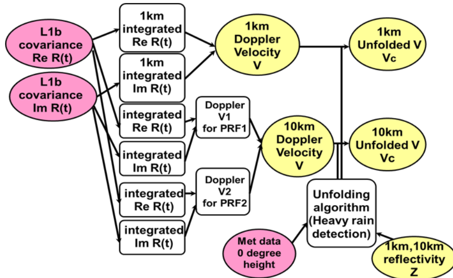
Figure 3.1.1.2.1-5 Processing flow of 1-km and 10-km averaged Doppler velocity
