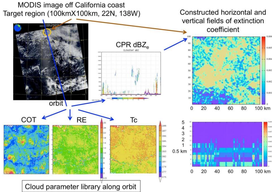
Fig. 4.4.3. A method of constructing a 3D extinction coefficient field from CPR and imager data. CLOUDSAT and AQUA MODIS cases on July 2, 2007.
