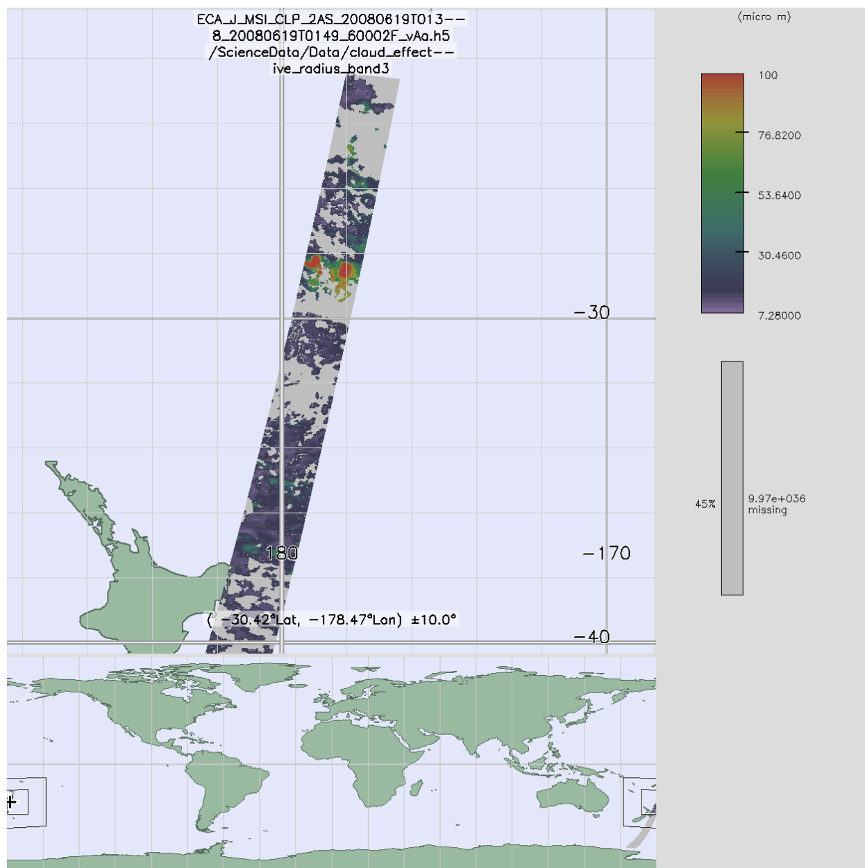
Fig.3.3.2.2.1.2 A sample of cloud effective radius from L2A cloud product, which contains both water and ice clouds.
