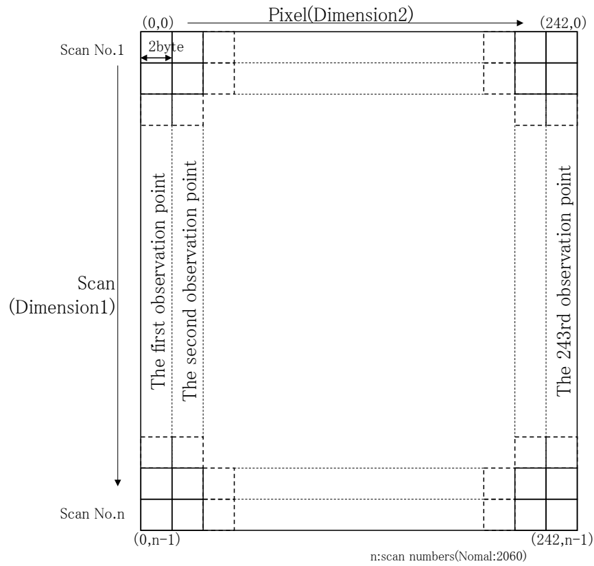
Figure 3-7 EarthAzimuth_P89o, EarthIncidence_P89o, SunAzimuth_P89o, SunElevation_P89o
