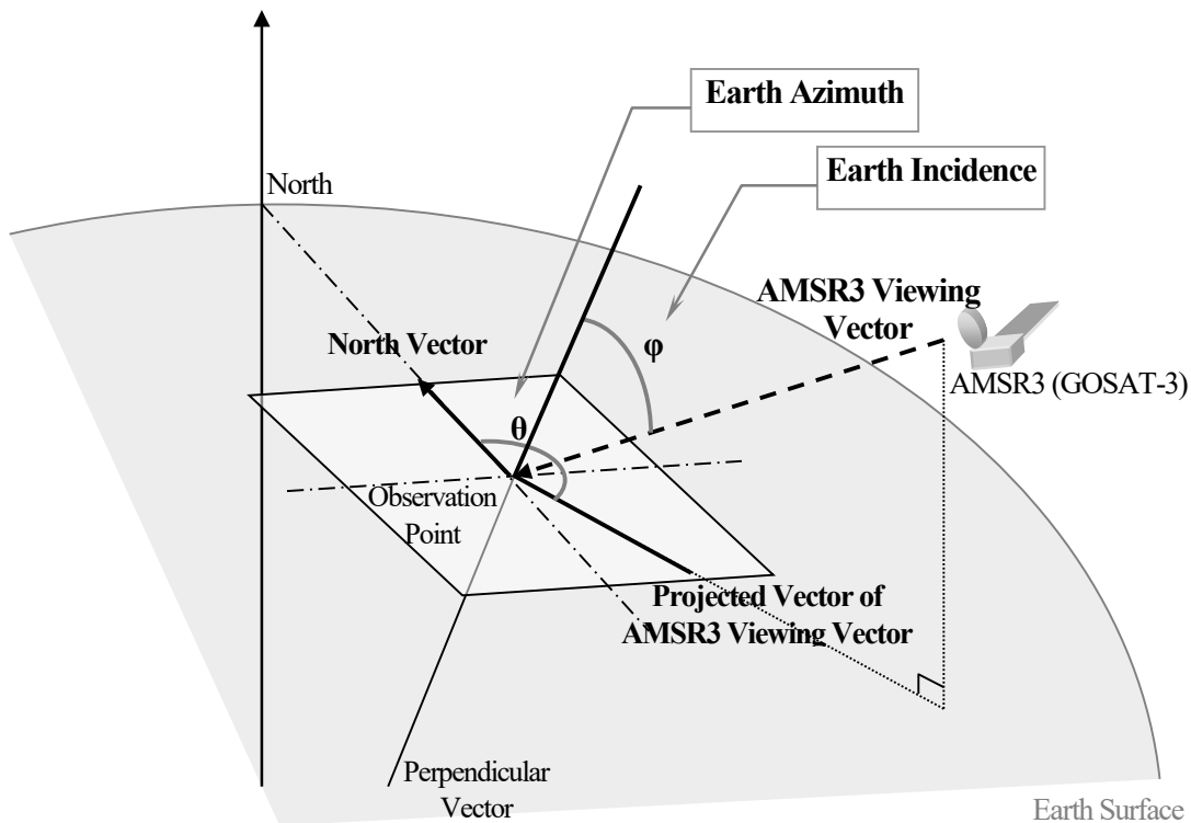
Figure 4-2 The definition of Earth Azimuth,Earth Incidence
