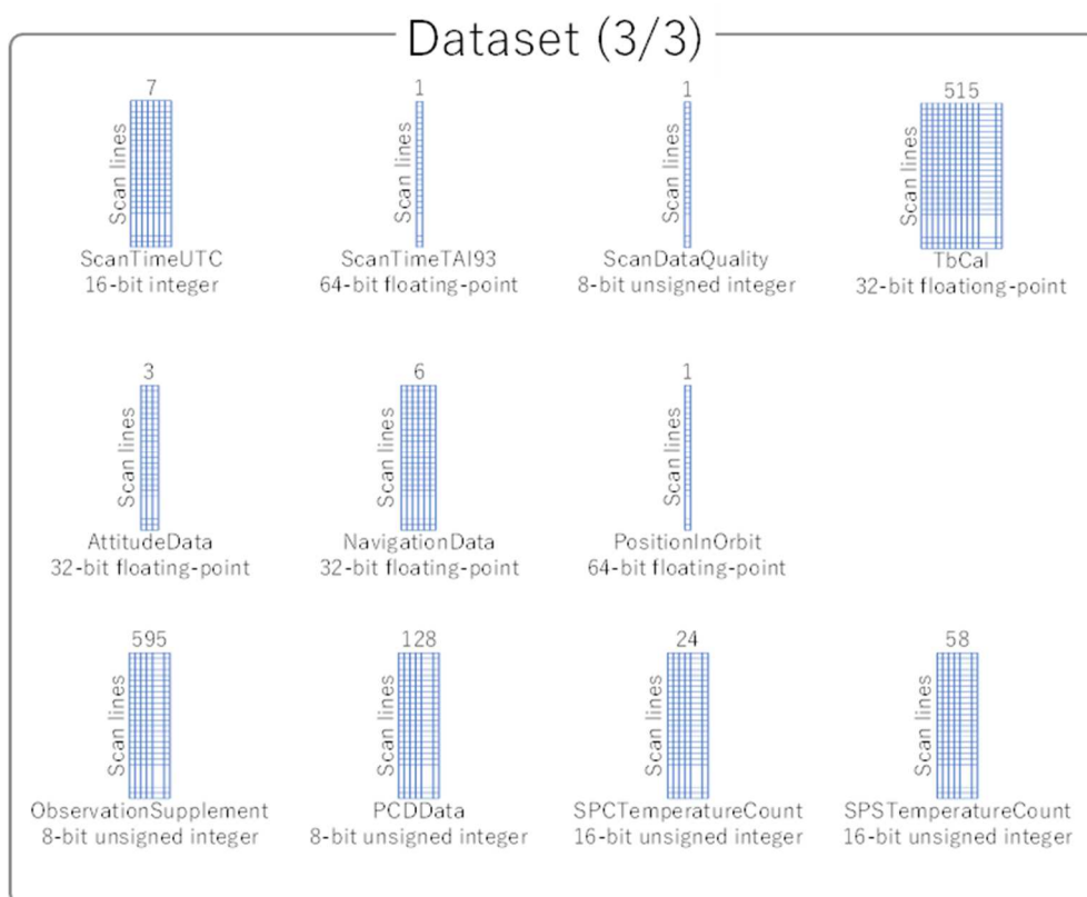
Figure 3-3 Structure of L1A product (3/3)
