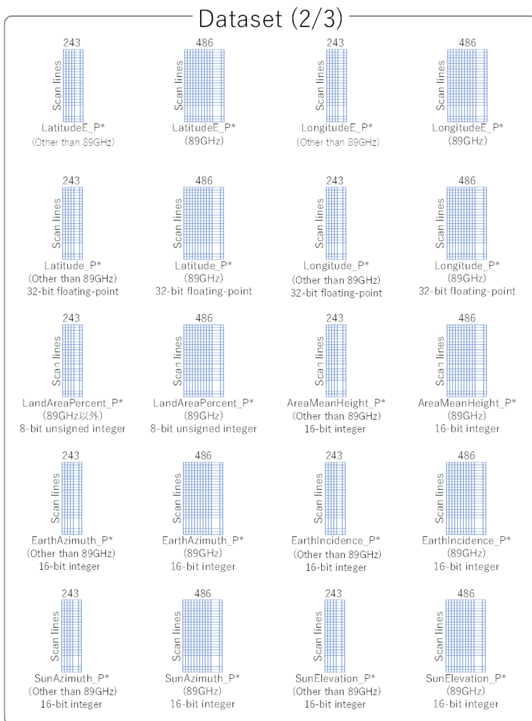
Figure 3-2 Structure of L1A product (2/3)
