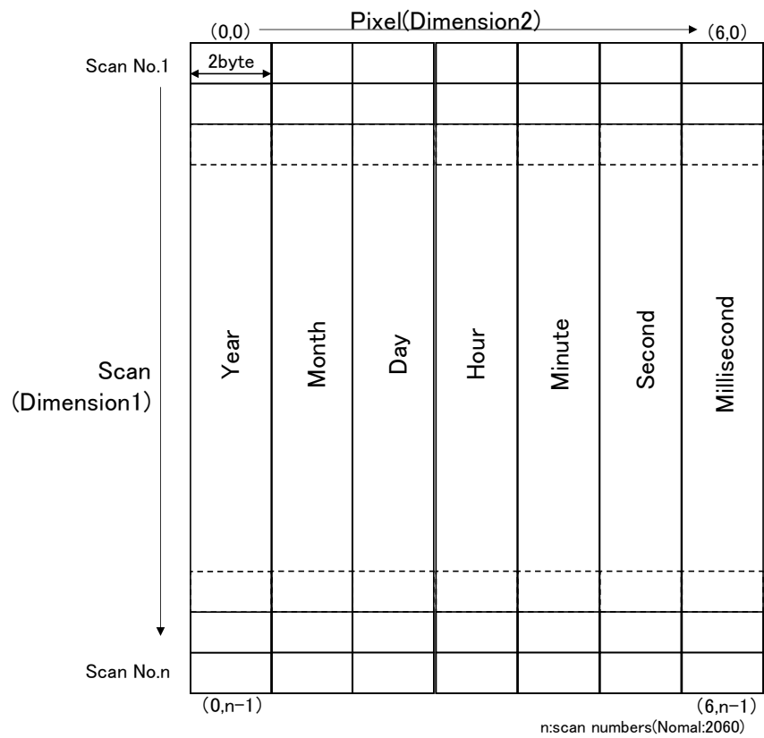
Figure 3-20 ScanTimeUTC
