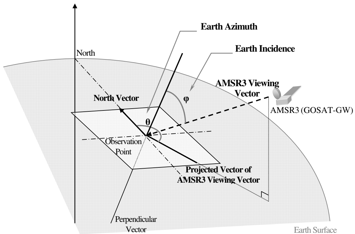
Figure 4-1 The definition of Earth Azimuth,Earth Incidence
