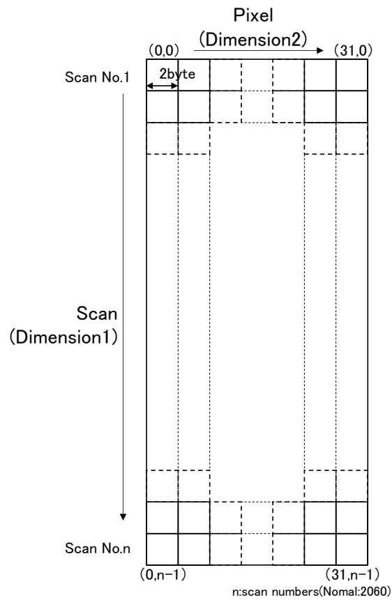
Figure 3-6 CSMCount(89GHz), HTSCount(89GHz)
