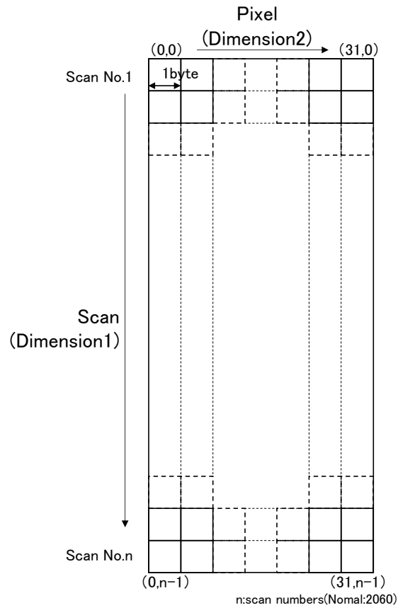
Figure 3-8 CSMCount_Quality(89GHz), HTSCount_Quality(89GHz)
