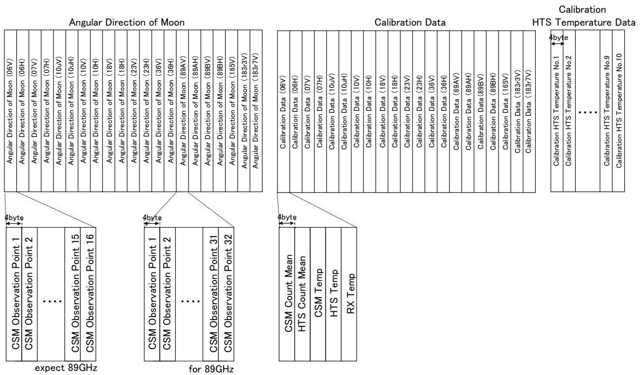
Figure 3-24 TbCal Details (Dataset Name : TbCal)
