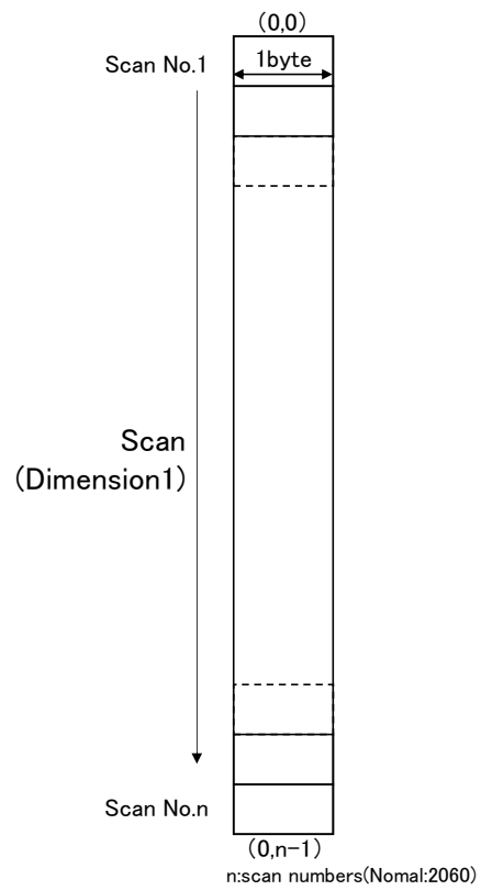
Figure 3-22 ScanDataQuality (Dataset Name : ScanDataQuality)
