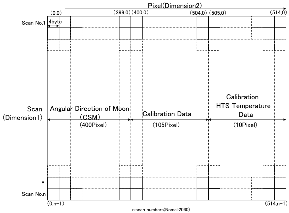
Figure 3-23 TbCal (Dataset Name : TbCal)
