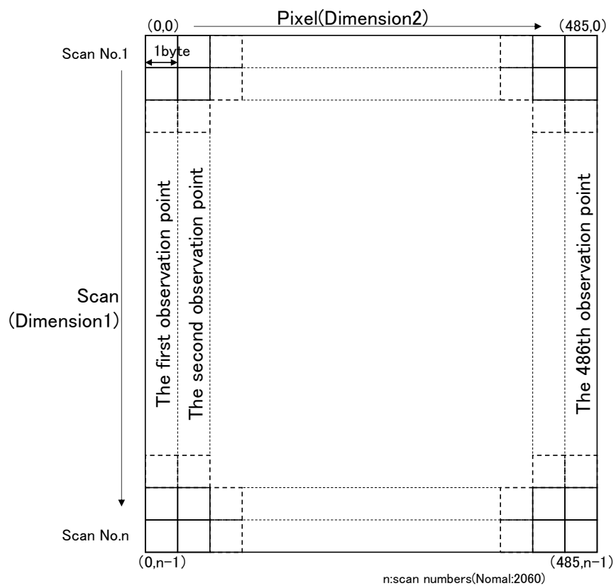
Figure 3-10 ObsCount_Quality (89GHz)
