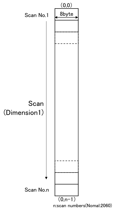
Figure 3-27 PositionInOrbit
