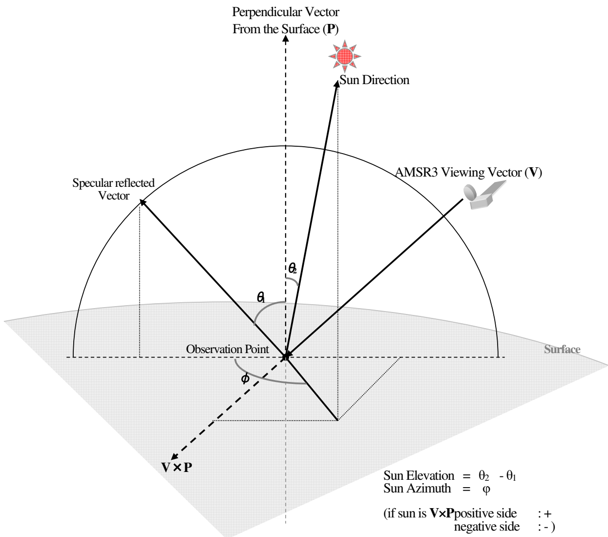
Figure 4-3 Definition of sun elevation angle and sun azimuth angle
