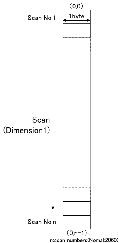
Figure 3-11 RxOffsetCount, RxGainCount
