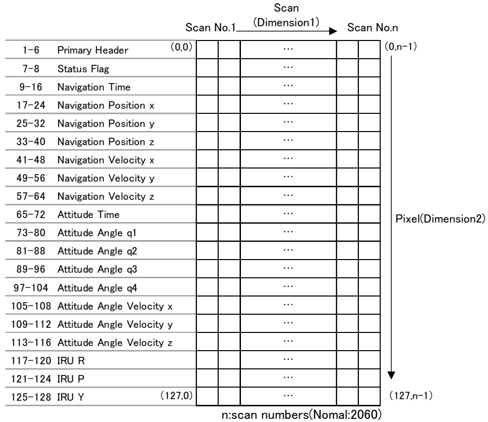
Figure 3-29 PCDData (Dataset Name : PCDData)
