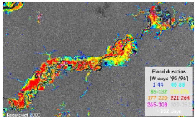
Figure 5. Flood duration map (Jaú river, AM/Brazil) derived from a time-sequence of 9 consecutive JERS-1 SAR scenes, acquired during one flood cycle Oct. 1995 - Oct. 1996. © NASDA/METI
