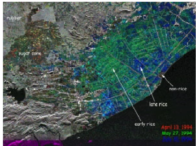
Figure 4. Irrigated rice (Perlis, Malaysia). Multi-temporal JERS-1 SAR. Rice paddy can be distinguished from other land use/land cover classes through its characteristic temporal signature. Local variations in the crop cycle are visible as green and blue. © NASDA/METI
