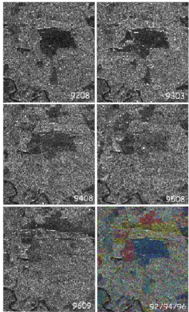
Figure 3. Monitoring of forest change (Kedah, Malaysia). Clear felling and regeneration patterns visible in the 4-year JERS-1 SAR time sequence. © NASDA/METI
