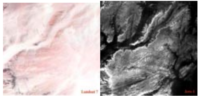
Figure 6. Mapping of sub-surface geology with SAR. LANDSAT ETM+ quick-look mosaic (left) , JERS-1 SAR "SAHARASAR" mosaic (right).
