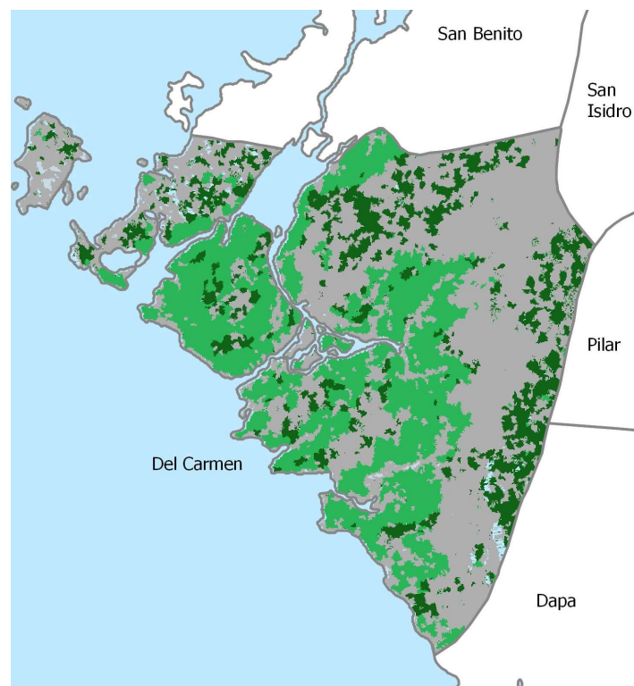
Extra Trees Classifier Mangrove Cover 2017
