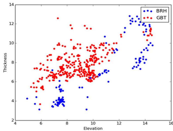
Thickness vs. 2011 LiDAR elevation (m)
