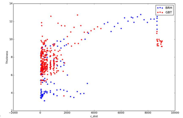
Thickness vs. Distance From nearest canal (m)
