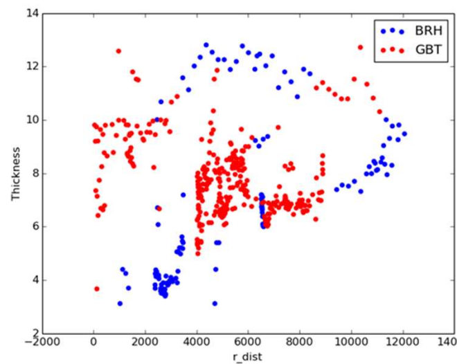
Thickness vs. Distance From nearest river (m)
