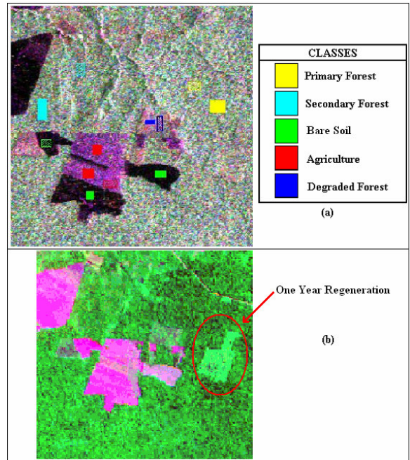
Figure 2 . a) PLR image (2006, October 21), composition: HH-VH-VV on RGB and b) TM Landsat-5 composition:5-4-3on RGB (2006, August 21). Degraded areas are only distinctly visible in PALSAR while One Year Regeneration is only noticeable in TM composition.
