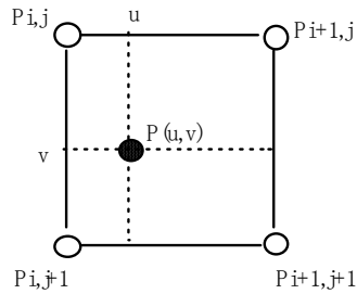
Bi-linear
