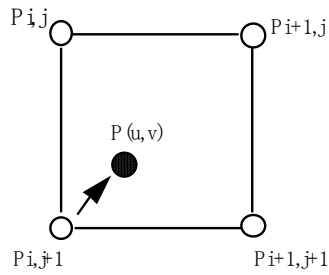
Nearest neighbor
