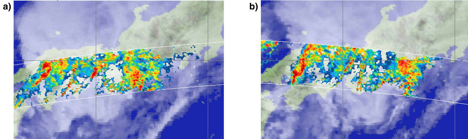
Fig.1 Horizontal cross section of rain at 2.0km height
