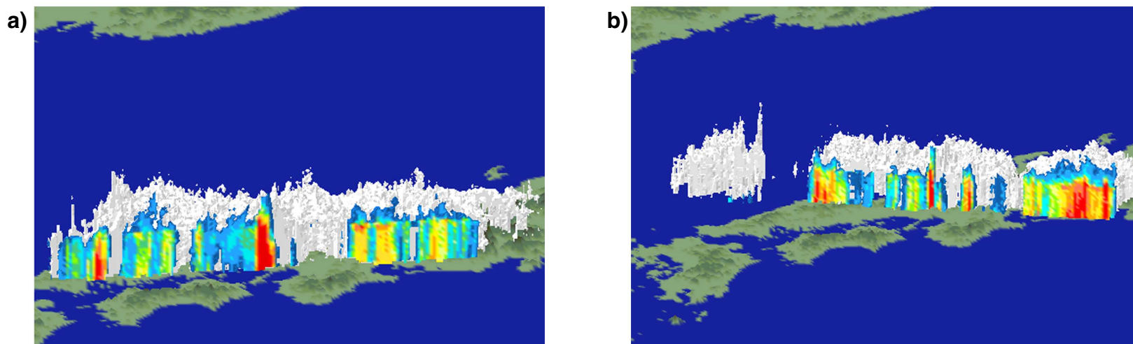
Fig.2 Three-dimensional Image of precipitation
