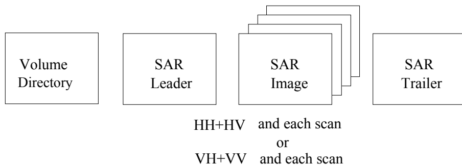
Figure 3.1-4 CEOS level 1.1(Scan SAR)/1.5/3.1 file composition/Dual polarization
